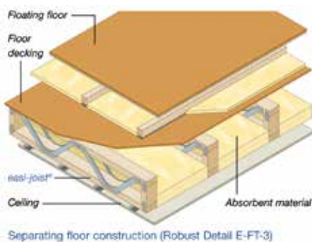
E-FT-3 Separating Floor – Metal Web Joists Use with Timber Frame walls only
